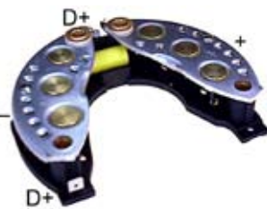
131569 Rectifier Replacing: UBB242, UBB240 Diode Amp. 50, O.D. 116.00, I.D. 37.10 w/ Diode Trio. 82 Ohm. Resistor.
