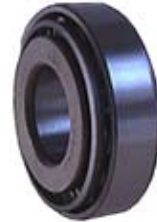
140803 Roller Bearing Replacing: 1900910202 O.D. 47.00, I.D. 40.00, H. 15.30
