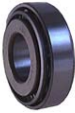
140803 Roller Bearing O.D. 47.00, I.D. 40.00, H. 15.30
